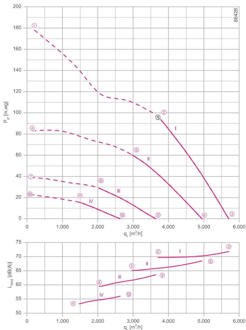
Characteristic curve
